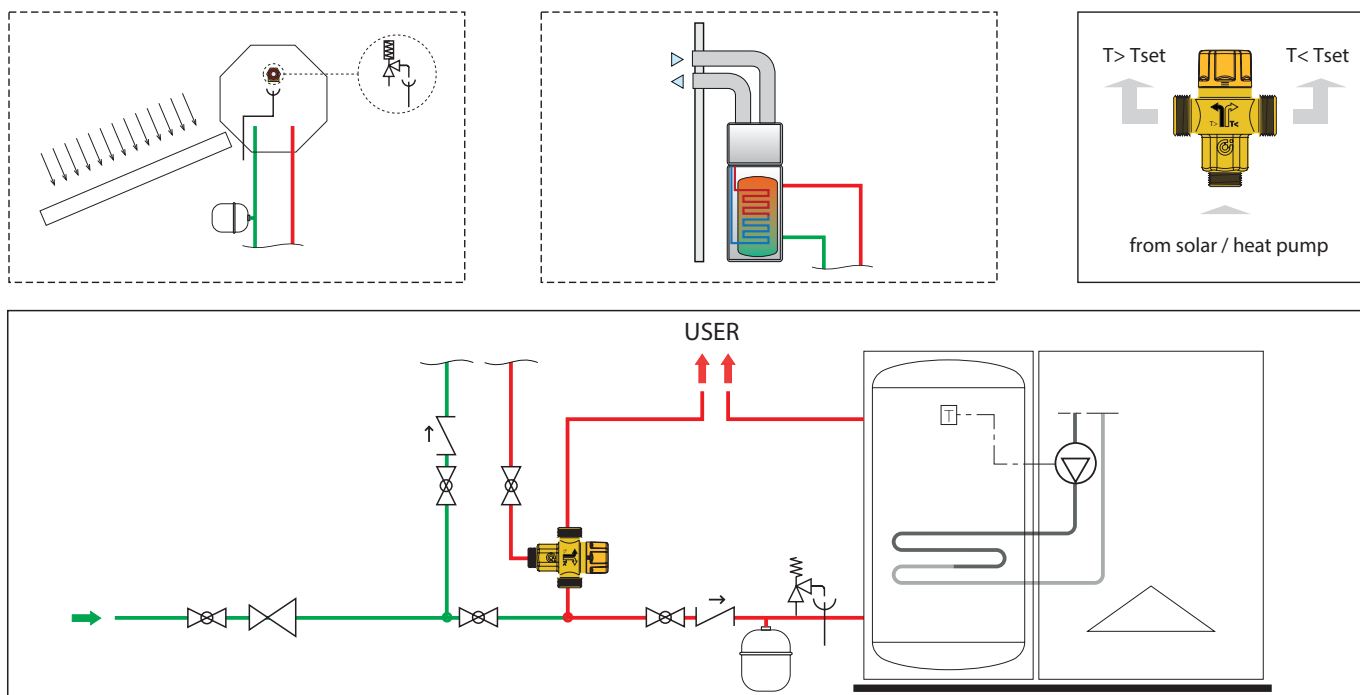
2620 series thermostatic diverter valve application diagram
