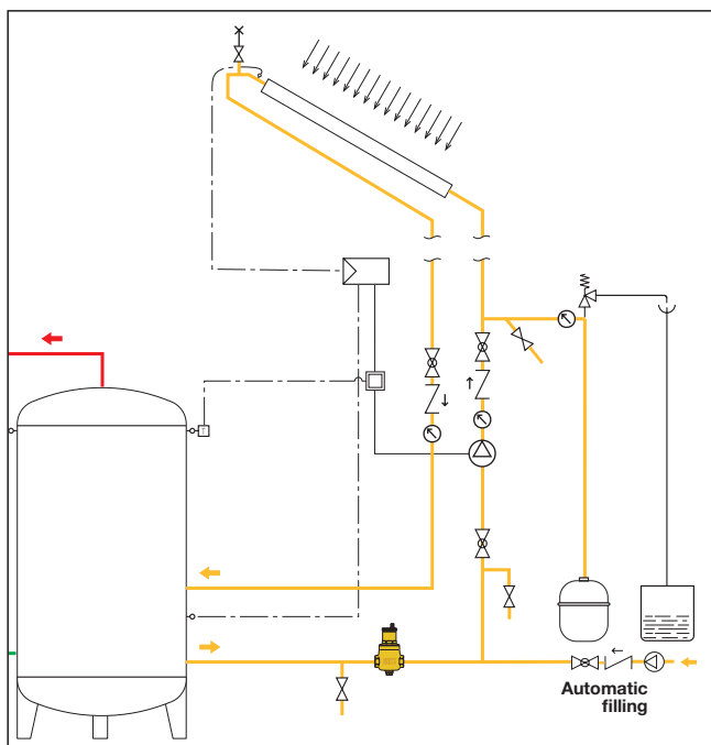
Application diagram for DISCAL® vertical 251 series
