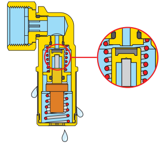
Opened position
