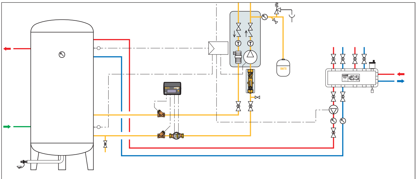
Application diagram for 75025 series heat meter and 258 series balancing valve
