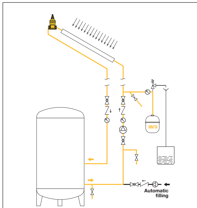
Application diagram, 251 series
