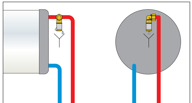
Application diagram for 603 series device on domestic water circuit
